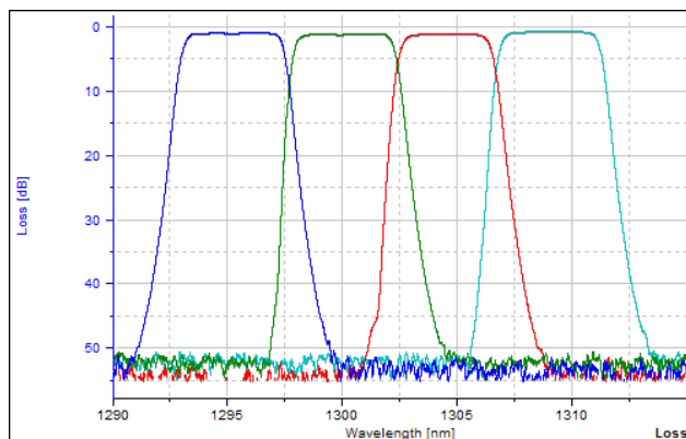
Sample measurement of an LR4-ROSA device
